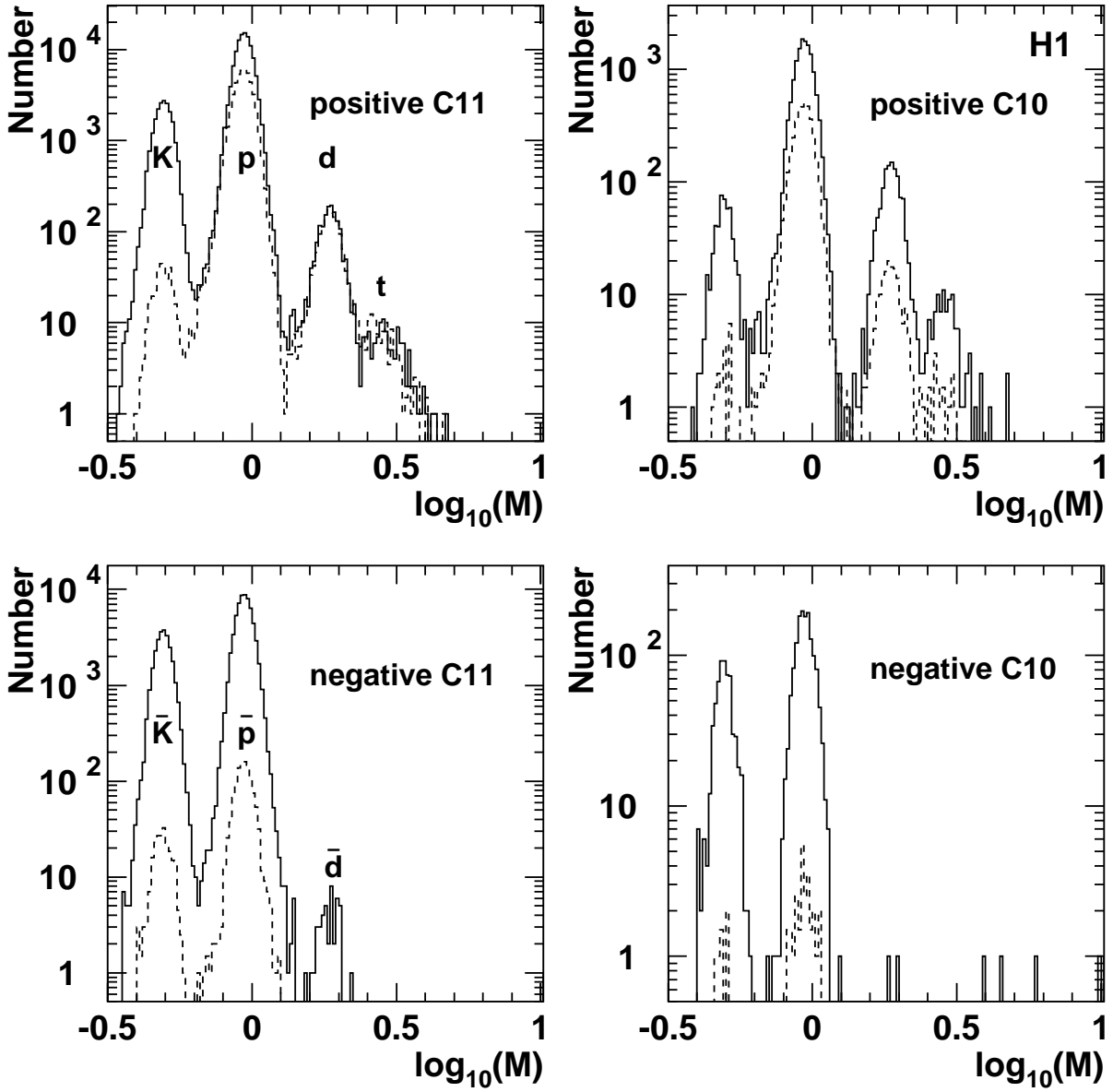
Figure 4: The mass spectra (with M in GeV) for positive and negative particles in the hard selected sample for the mainly photoproduction ( C_{11} ) and mainly pG ( C_{10} ) samples. The dashed lines show the material background deduced from the sideband subtraction method.
