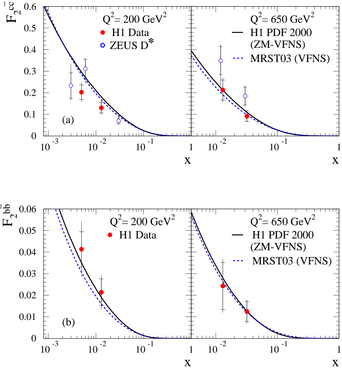
Figure 8: The measured F_2^{c\bar{c}} (a) and F_2^{b\bar{b}} (b) shown as a function of x for two different Q^2 values. The inner error bars show the statistical error, the outer error bars represent the statistical and systematic errors added in quadrature. The F_2^{c\bar{c}} from ZEUS obtained from measurements of D^* mesons [2] and the predictions of NLO QCD fits [16, 31] are also shown.
