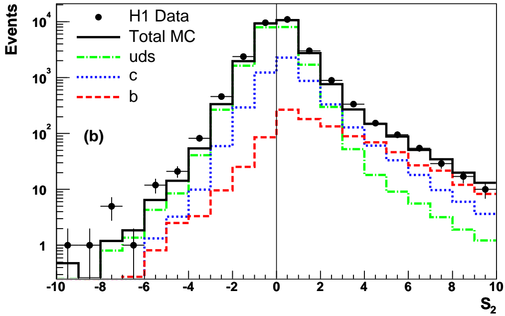
Figure 5: The significance S_1 = \delta/\sigma(\delta) distribution per event (a) for events that contain one reconstructed CST track associated to the jet axis and the significance S_2 = \delta/\sigma(\delta) distribution per event (b) of the track with the second highest absolute significance for events with \geq 2 reconstructed CST tracks associated to the jet. Included in the figure is the expectation from the RAPGAP Monte Carlo simulation, showing the contributions from the various quark flavours after applying the scale factors obtained from the fit to the subtracted significance distributions of the data.
