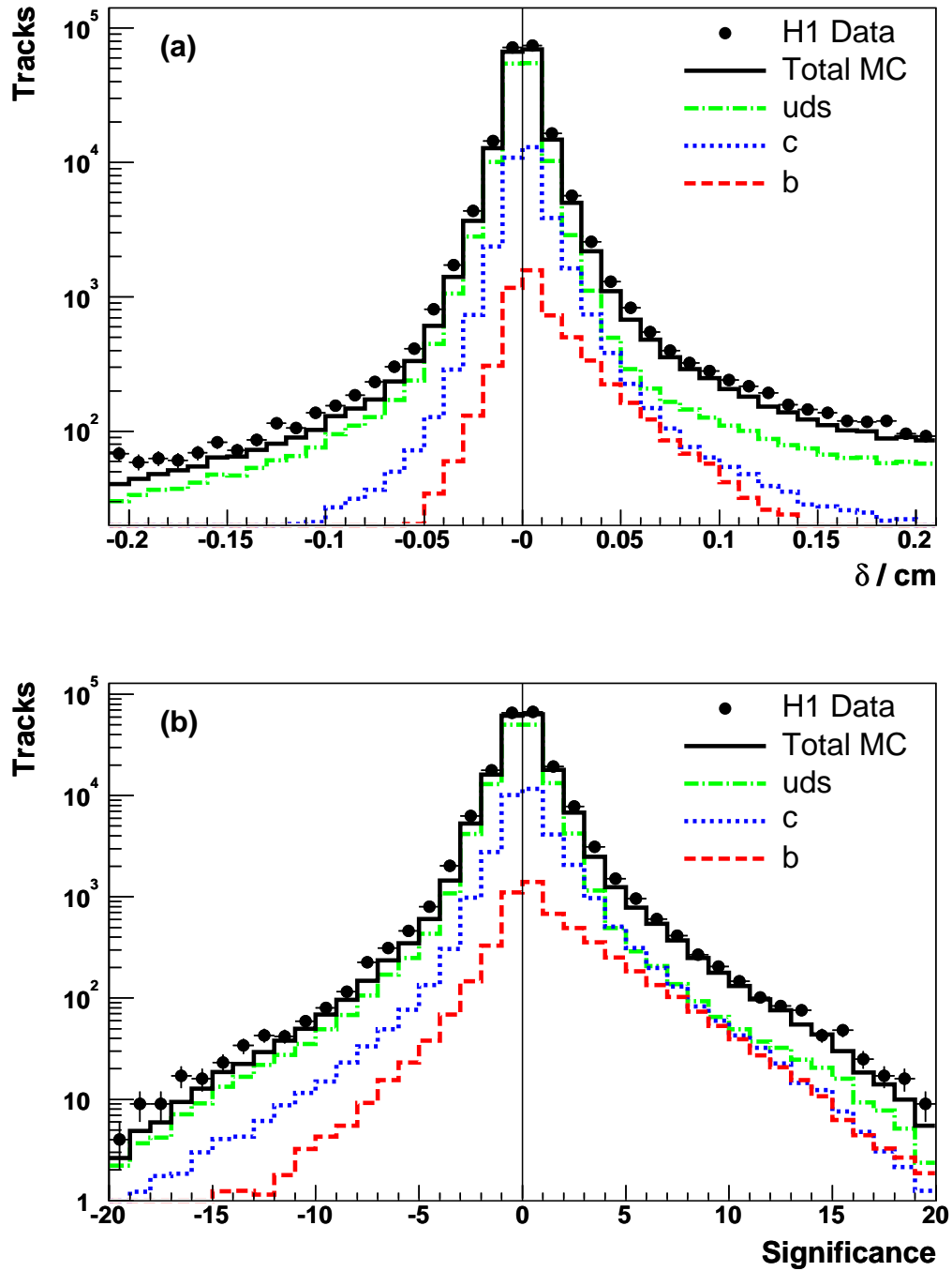
Figure 4: The signed impact parameter \delta of a track to the primary vertex in the x - y plane (a) and the significance \delta/\sigma(\delta) (b), where \sigma(\delta) is the error on \delta , for all CST tracks associated to the jet axis. The cut |\delta| < 0.1 cm has been applied in figure (b). Included in the figure is the expectation from the RAPGAP Monte Carlo simulation, showing the contributions from the various quark flavours after applying the scale factors obtained from the fit to the subtracted significance distributions of the data.
