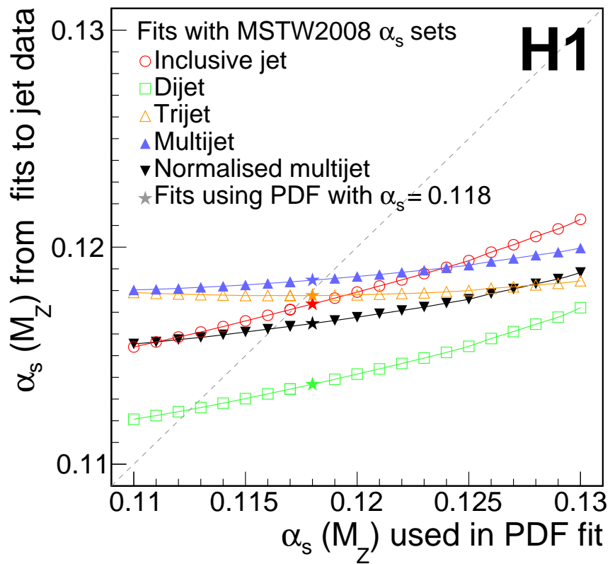
Figure 18: Values of \alpha_s(M_Z) extracted from fits of the NLO QCD predictions to the jet cross section measurements. Shown are the values of \alpha_s(M_Z) obtained with the inclusive jet, dijet and trijet data separately, and for fits either to the multijet or to the normalized multijet measurements. Each point stands for a value of \alpha_s(M_Z) obtained using a PDF set which has been determined assuming a fixed values of \alpha_s(M_Z) as indicated.
