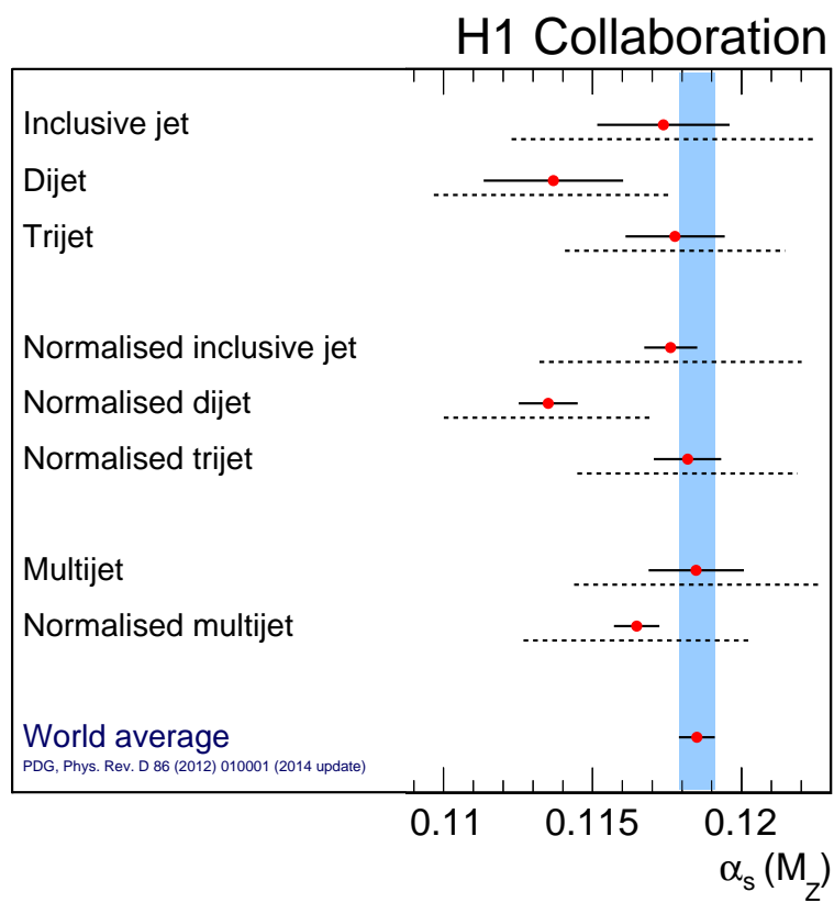
Figure 20: Comparison of \alpha_s -values extracted from different jet cross section measurements, separately and simultaneously, to the world average value of \alpha_s(M_Z) . The full line indicates the experimental uncertainty and the dashed line the theoretical uncertainty. The band indicates the uncertainty of the world average value of \alpha_s(M_Z) .
