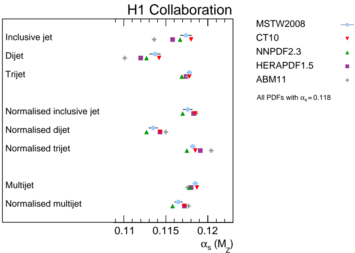
Figure 19: Values of \alpha_s(M_Z) extracted from fits of NLO QCD predictions to the absolute and normalised jet cross sections using different PDF sets: MSTW2008, CT10, NNPDF2.3, HERAPDF1.5 and ABM11. For the MSTW2008 PDF set the PDF uncertainty on \alpha_s(M_Z) as determined from the MSTW2008 eigenvectors is shown as horizontal error bar.
