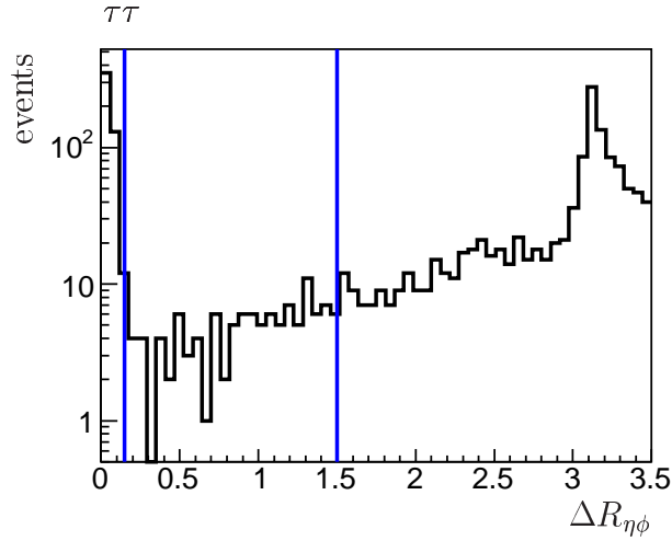
Figure 4.7: \eta\phi -Distance between \tau -jet candidates and their closest track. The vertical lines denote the inner and outer cone.
