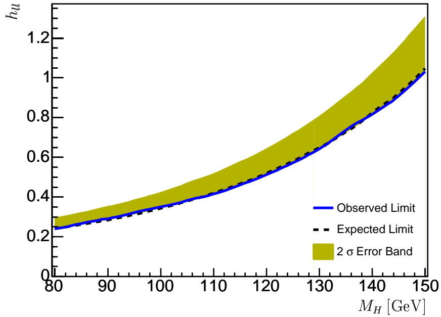
Figure 5.11: 95% CL limit on the diagonal coupling h_{ll} as determined from the \tau\tau selection. The democratic assumption BR(H^{++} \rightarrow ee/\mu\mu/\tau\tau) = 33\% is made in this plot.
