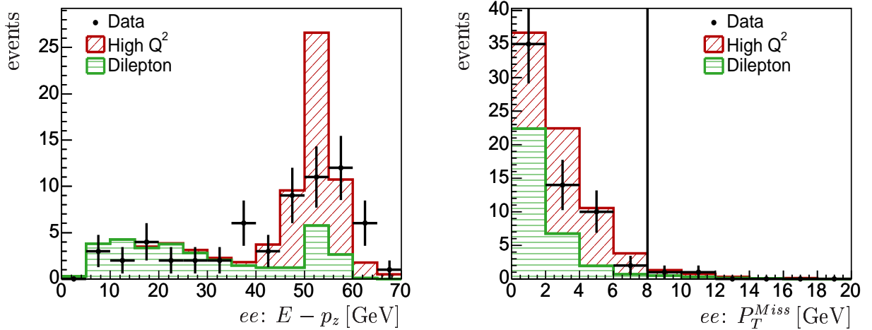
Figure 4.5: E - p_z (left) and P_T^{Miss} (right) distributions for the ee event class ( e\tau topology) for the 99/00 dataset after preselection. The vertical line in the P_T^{Miss} spectrum denotes the cut position.
