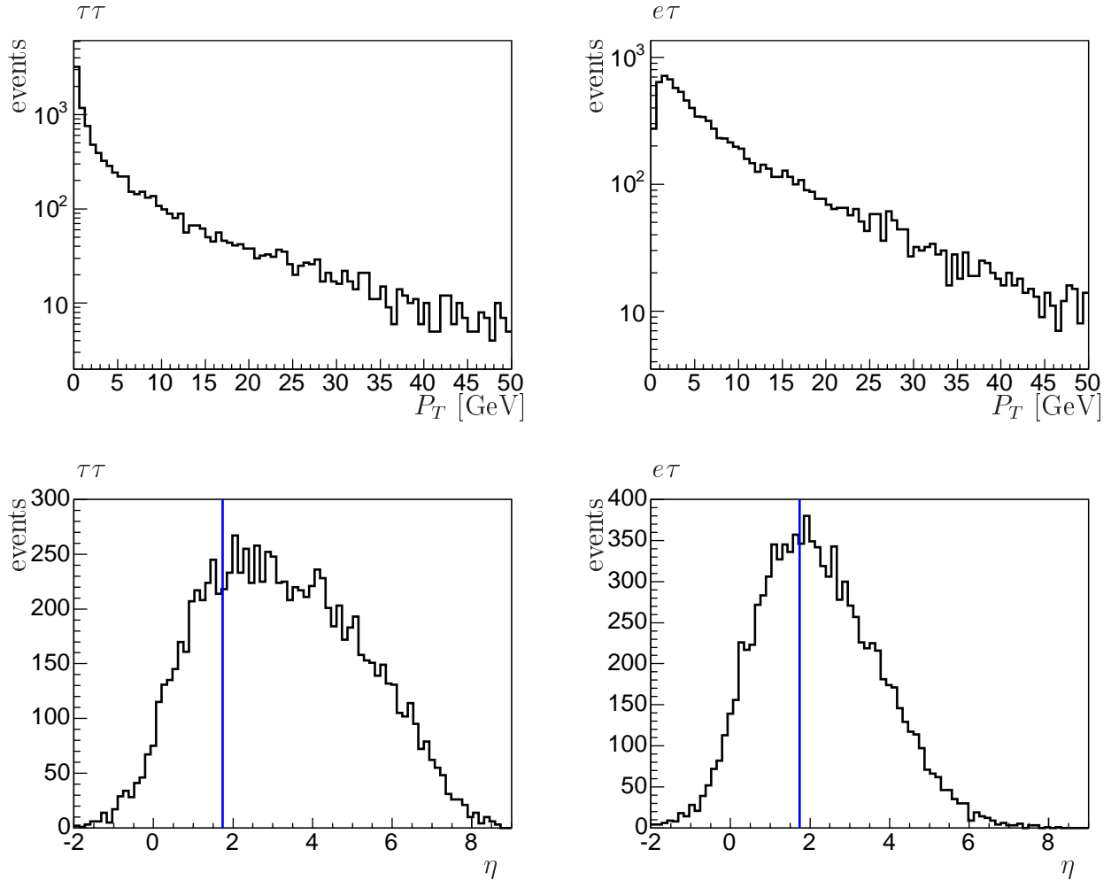
Figure 3.3: Generator level P_T (upper) and \eta (lower) spectra of the pseudoscattered lepton for \tau\tau (left) and e\tau (right). The vertical bar in the \eta distributions denotes the forward boundary of the central region, in which the candidates are required to be.
