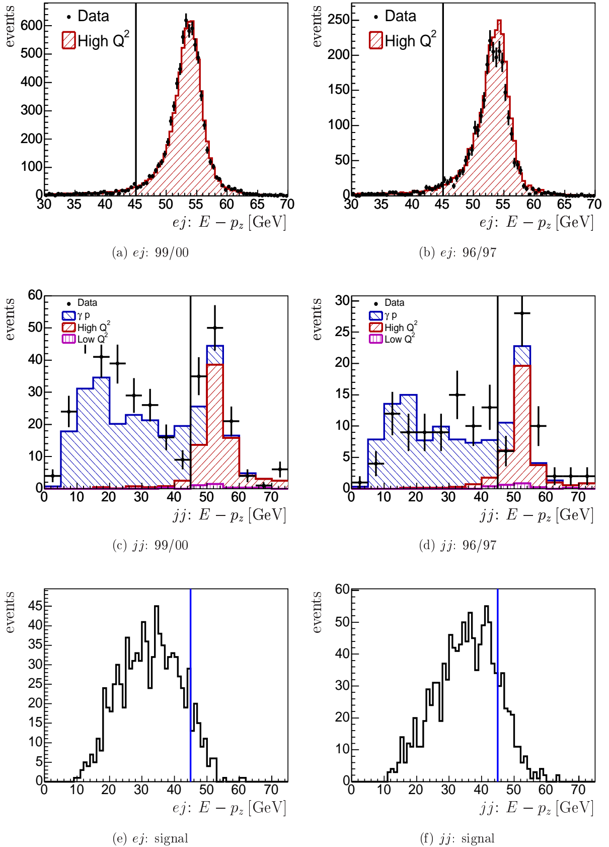
Figure 4.1: E - p_z distributions for the ej and jj event classes for data and background, as well as for a signal MC of a 100 GeV Higgs. The normalisation mismatch in jj for 99/00 and ej for 96/97 can be clearly seen. The vertical line denotes the cut position.
