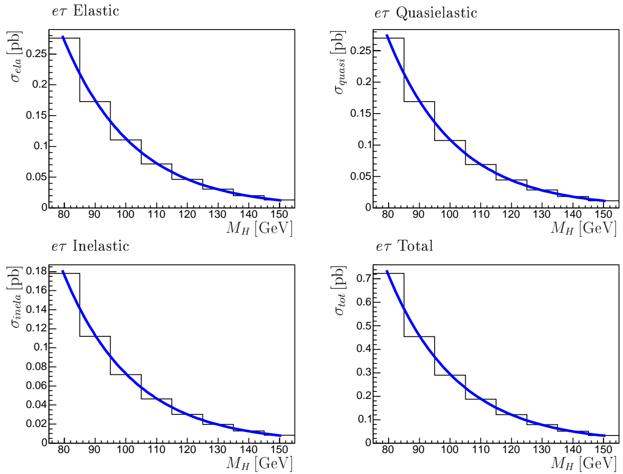
Figure 1.7: Same distributions as shown in Figure 1.6 but with the coupling constant h_{e\tau} = 0.3 . All other couplings are assumed zero.
