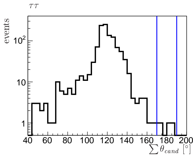
Figure 3.6: \sum \theta of the candidates for a \tau\tau signal MC of a 100 GeV Higgs. The region enclosed by the vertical bars is cut away.
