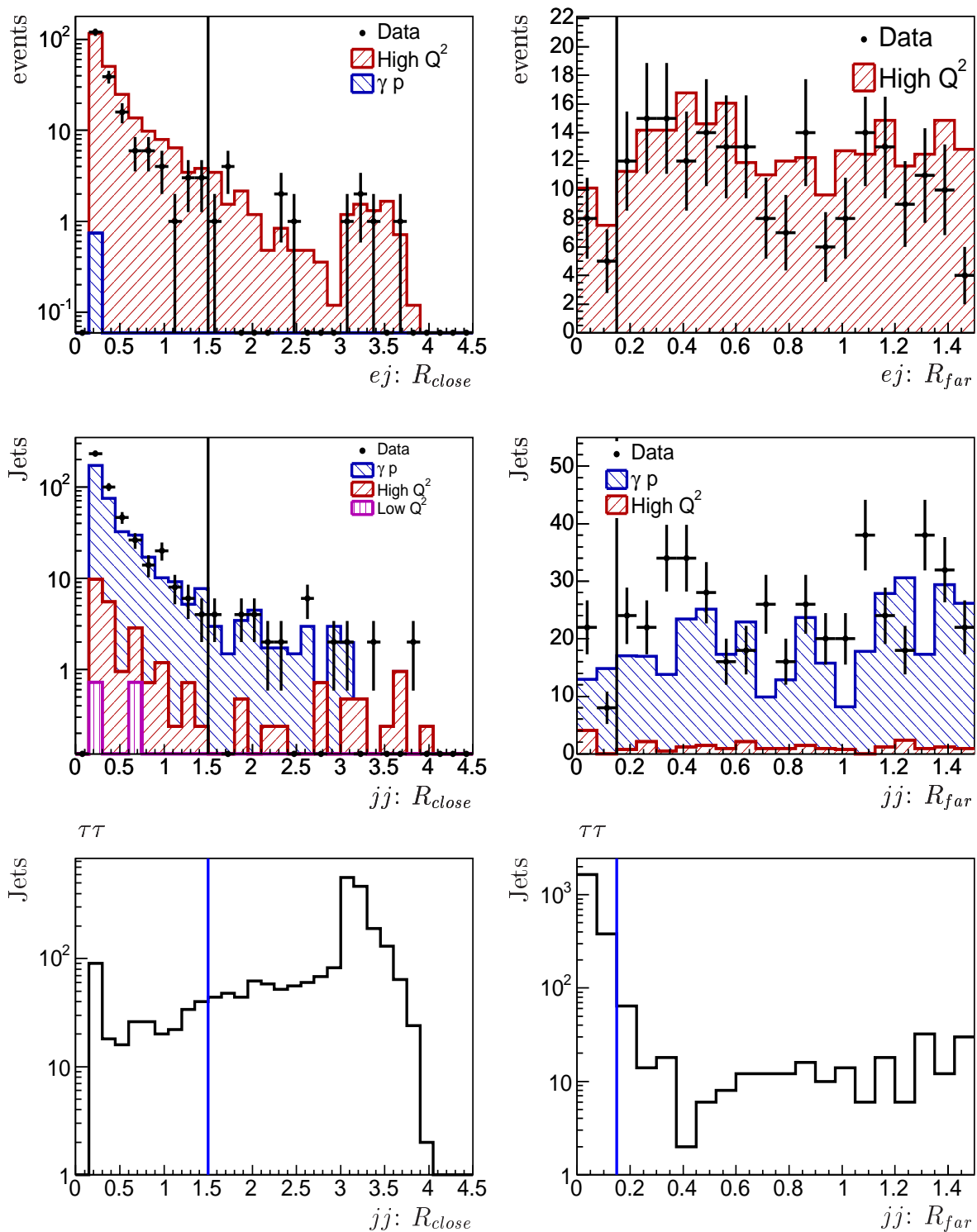
Figure 4.8: Jet isolation variables R_{close} and R_{far} as described in the text for the ej (top) and jj (middle and bottom) event classes. For jj both jets enter the plots, therefore the number of events is half the number of jets. Events/jets to the left (right) of the vertical line in the R_{close} ( R_{far} ) distribution are rejected. From the signal distributions (bottom plots, 100 GeV Higgs) it becomes clear that the bulk of the events/jets survives.
