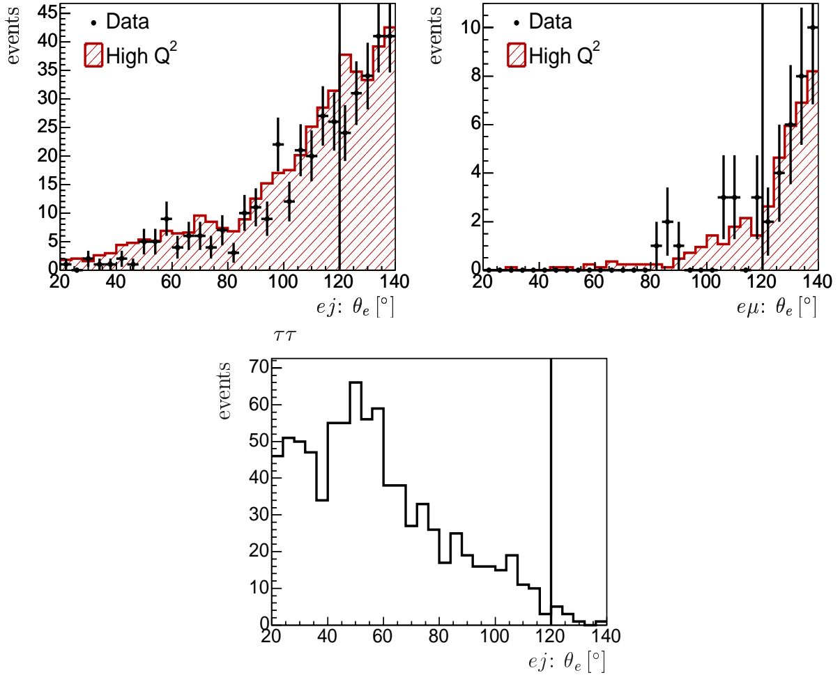
Figure 4.6: \theta_e for the e_j (top left) and e_\mu (top right) event classes for \tau\tau . The vertical line denotes the cut position. The cut removes a considerable amount of background but only a small amount of signal events (bottom) as shown for the case of a 100 GeV signal. The signal distribution for other event classes is analogue.
