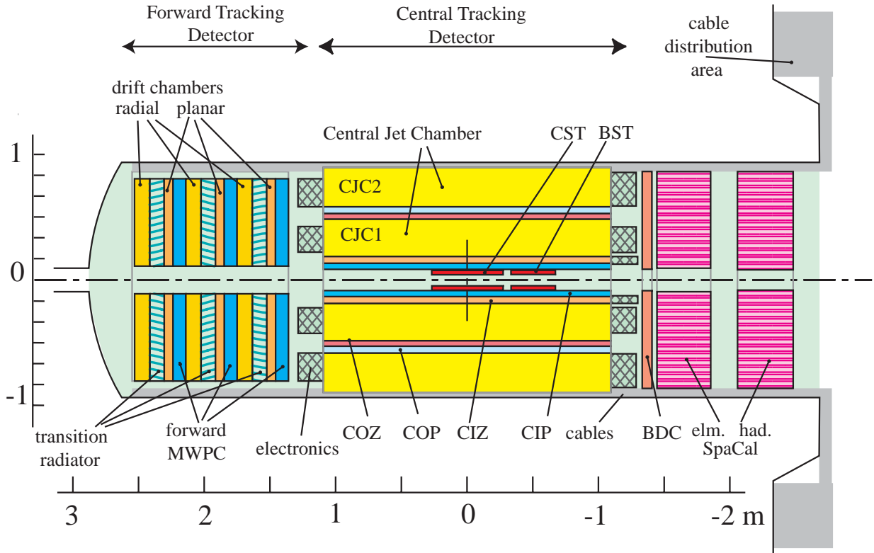
Figure 2.3: Side view of the H1 tracking system.
