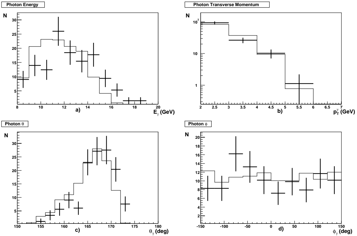
Figure 4.11: The full event sample distributions, a) energy of the final photon in the SpaCal, b) the transverse momentum of the photon, c) the polar \theta distribution and d) the azimuthal \phi of the photon. The data (crosses) are compared to the HERWIG prediction (solid lines).
