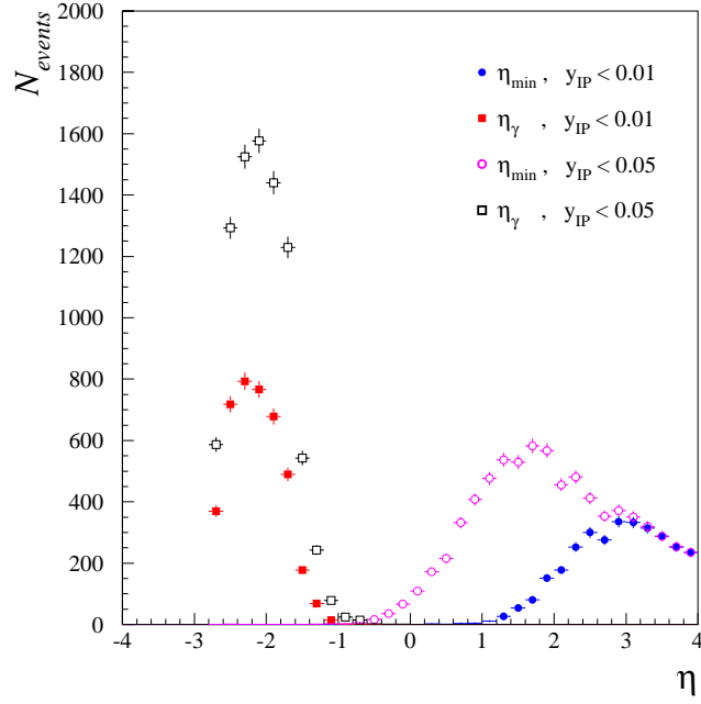
Figure 4.5: The rapidities of the final photon and the backward edge of the proton dissociation system Y for two different y_{\mathcal{P}} cuts. (taken from [20])
