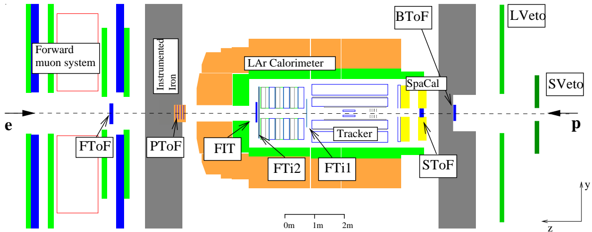
Figure 3.9: The H1 Time-of-Flight system, including all the devices installed after the HERA-II upgrade, when additional ToF systems was installed, namely the FTi1 in between the central and the forward tracker, operating together with the FTi2, a scintillator system between the forward tracker and the inner forward section of the LAr calorimeter.
