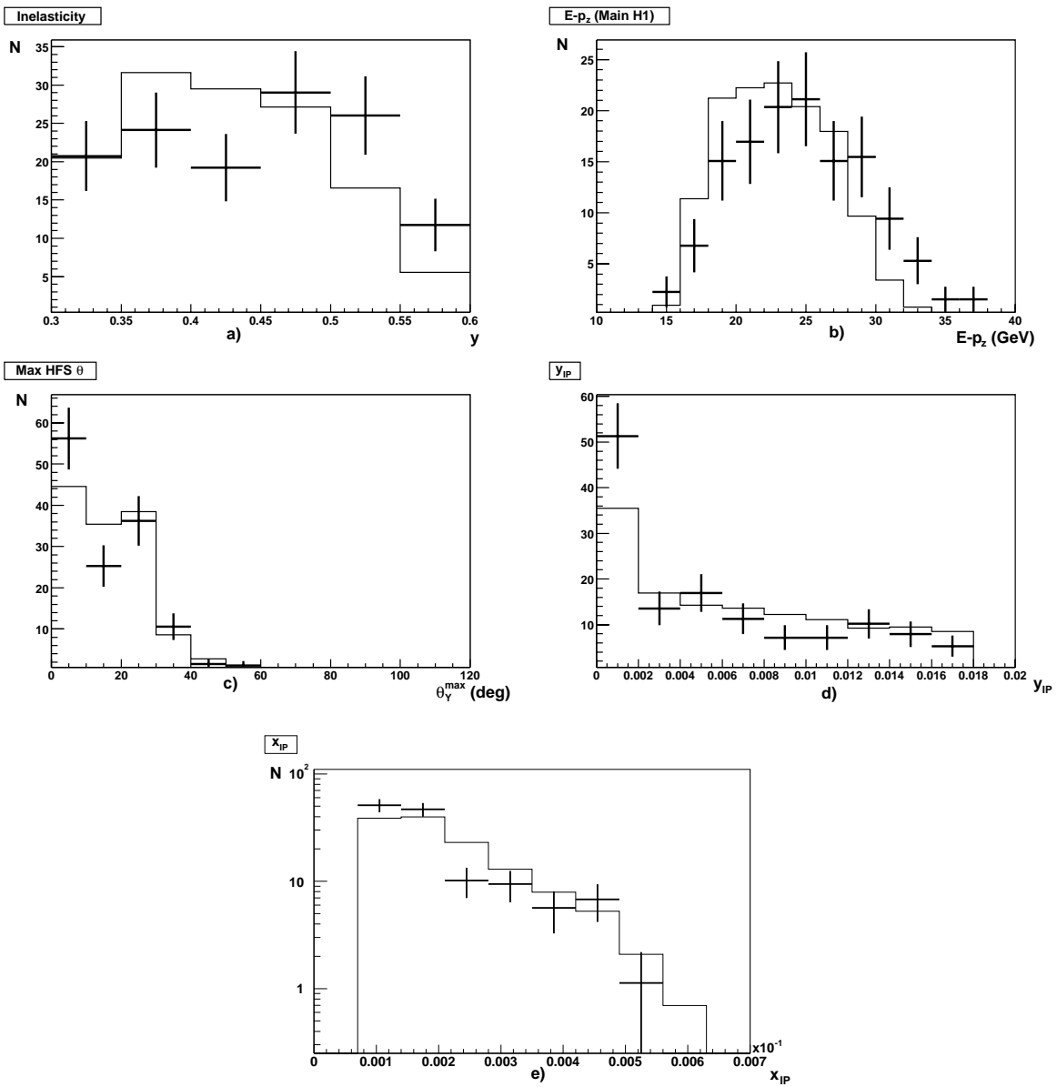
Figure 4.12: The full event sample distributions, a ) the inelasticity y , b ) the E - p_z of the main H1 detector, c ) the maximum polar angle of the HFS particles of the proton dissociation, d ) the y_{IP} variable and e ) the x_{IP} variable. The data (crosses) are compared to the HERWIG prediction (solid lines).
