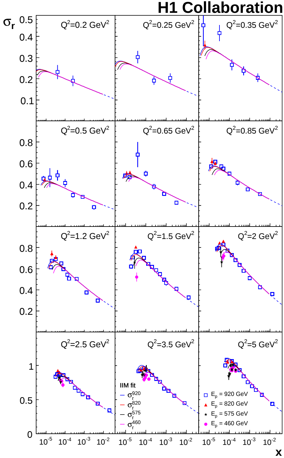
Figure 26: Reduced cross-section data taken at different proton beam energies E_p compared to IIM fit results for 0.2 \leq Q^2 \leq 5 \text{ GeV}^2 .
