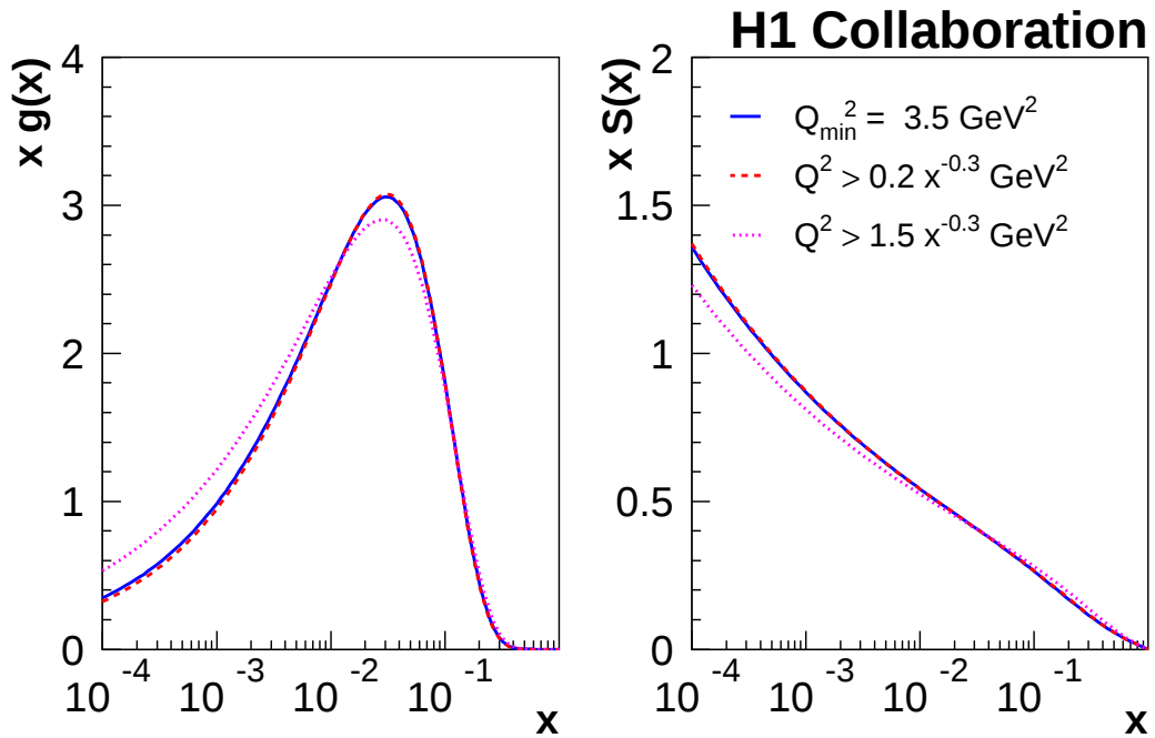
Figure 25: Gluon and sea quark PDFs shown at the starting scale Q_0^2 = 1.9 \text{ GeV}^2 for the central fit with Q_{\min}^2 = 3.5 \text{ GeV}^2 and for the fits with additional cuts Q^2 > A_s x^{-0.3} where A_s = 0.2 and A_s = 1.5 .
