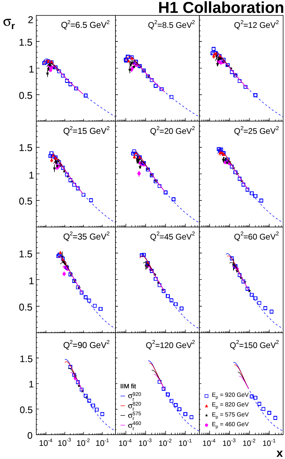
Figure 27: Reduced cross-section data taken at different proton beam energies E_p compared to IIM fit results for 6.5 \leq Q^2 \leq 150 \text{ GeV}^2 .
