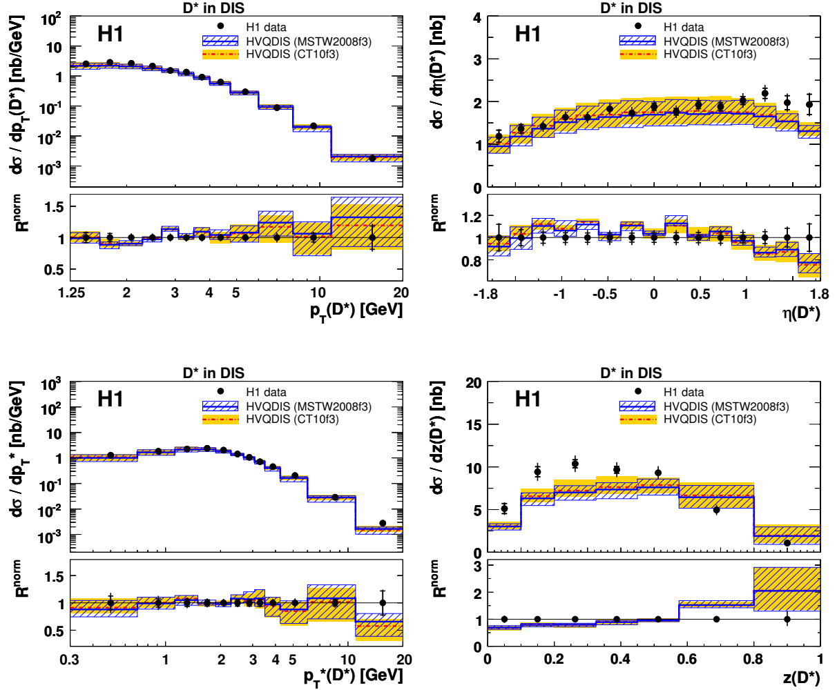
Figure 5: Differential D^* cross section as a function of the transverse momentum p_T(D^*) and pseudo-rapidity \eta(D^*) in the laboratory frame, the transverse momentum p_T^*(D^*) in the \gamma p centre-of-mass frame and the D^* inelasticity z(D^*) . The measurements correspond to the kinematic range of 5 < Q^2 < 100 \text{ GeV}^2 , 0.02 < y < 0.7 and |\eta(D^*)| < 1.8 and p_T(D^*) > 1.25 \text{ GeV} . The data are shown as points, the inner error bars show the statistical error, the outer error bars represent the statistical and systematic errors added in quadrature. The data are compared to predictions by the next-to-leading order calculation HVQDIS with two different proton parton densities. The bands indicate the theoretical uncertainties (table 2). In the lower part of the figures the normalised ratio R^{\text{norm}} of theory to data (equation 3) is shown, which has reduced normalisation uncertainties.
