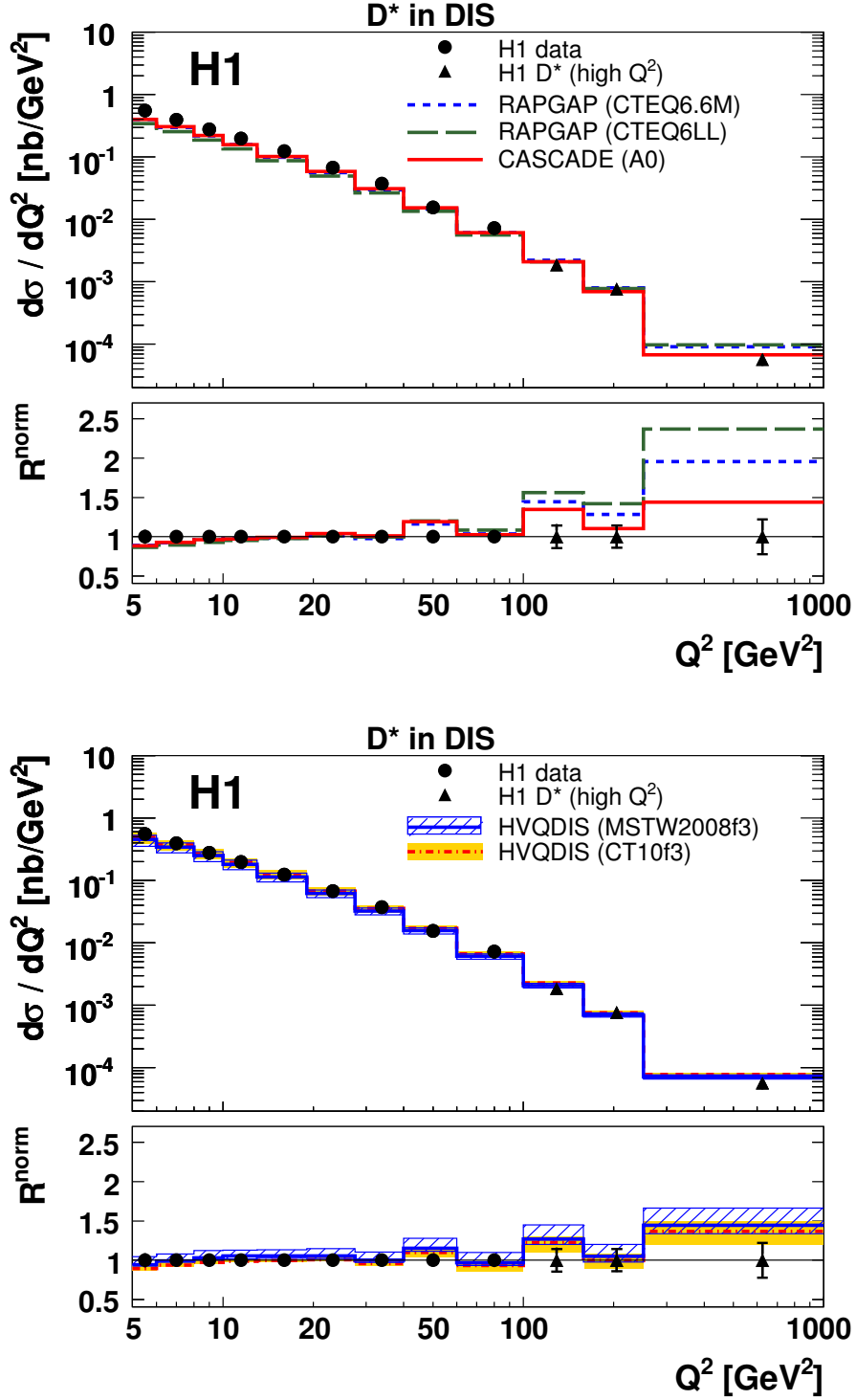
Figure 14: Differential D^* cross section as a function of the photon virtuality Q^2 . The measurements correspond to the kinematic range of 0.02 < y < 0.7 , |\eta(D^*)| < 1.5 and p_T(D^*) > 1.5 GeV. The data of this measurement (points) are shown in a phase space with stronger restrictions on \eta(D^*) and p_T(D^*) to be comparable to a previous measurement at higher Q^2 [15] (triangles). The inner error bars show the statistical error, the outer error bars represent the statistical and systematic errors added in quadrature. The data are compared to predictions by the MC program RAPGAP with two different proton PDFs and by the MC program CASCADE (left) and to predictions by the next-to-leading order calculation HVQDIS with two different proton PDFs (right).
