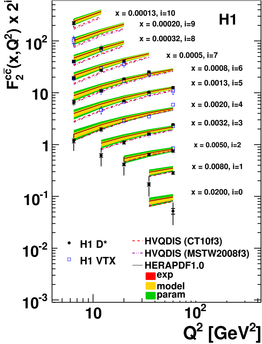
Figure 18: F_2^{c\bar{c}} as a function of Q^2 for different x , as derived from D^* data with HVQDIS (points). The inner error bars show the statistical uncertainty, the outer error bar the total uncertainty, including statistical, experimental systematic, extrapolation and model uncertainty added in quadrature. The data are compared to the measurement of F_2^{c\bar{c}} with the H1 vertex detector [14] (open squares), to NLO DGLAP predictions from HVQDIS with two different proton PDFs, and to the F_2^{c\bar{c}} prediction of HERAPDF1.0.
