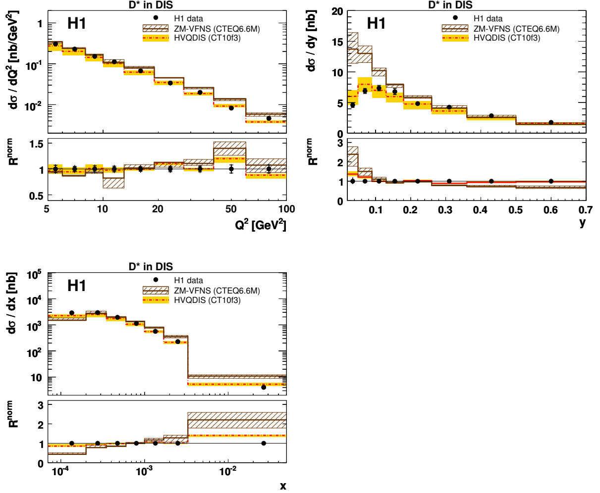
Figure 12: Differential D^* cross section as a function of photon virtuality Q^2 , the inelasticity y and Bjorken x . The measurements correspond to the kinematic range of 5 < Q^2 < 100 GeV ^2 , 0.02 < y < 0.7 , |\eta(D^*)| < 1.8 , p_T(D^*) > 1.25 GeV with an additional cut on the D^* transverse momentum in the \gamma p centre-of-mass frame p_T^*(D^*) > 2.0 GeV. The data are shown as points, the inner error bars show the statistical error, the outer error bars represent the statistical and systematic errors added in quadrature. The data are compared to a prediction to next-to-leading order in the ZM-VFNS and to HVQDIS. The bands indicate the theoretical uncertainties (table 2).
