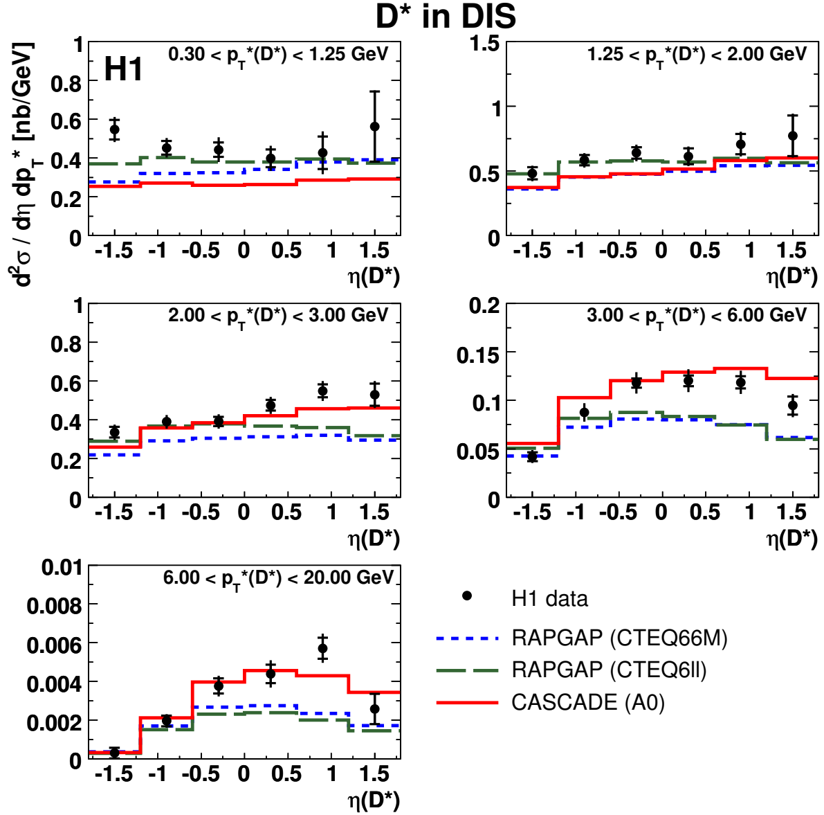
Figure 8: Double differential D^* cross section as a function of the transverse momentum in the \gamma p centre-of-mass frame p_T^*(D^*) and the pseudo-rapidity \eta(D^*) in the laboratory frame. The measurements correspond to the kinematic range of 5 < Q^2 < 100 GeV 2 , 0.02 < y < 0.7 and |\eta(D^*)| < 1.8 and p_T(D^*) > 1.25 GeV. The data are shown as points, the inner error bars show the statistical error, the outer error bars represent the statistical and systematic errors added in quadrature. The data are compared to predictions by the MC program RAPGAP with two different proton parton densities and by the MC program CASCADE.
