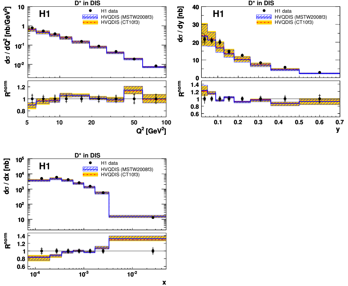
Figure 3: Differential D^* cross section as a function of the photon virtuality Q^2 , the inelasticity y and Bjorken x . The measurements correspond to the kinematic range of 5 < Q^2 < 100 \text{ GeV}^2 , 0.02 < y < 0.7 , |\eta(D^*)| < 1.8 and p_T(D^*) > 1.25 \text{ GeV} . The data are shown as points, the inner error bars show the statistical error, the outer error bars represent the statistical and systematic errors added in quadrature. The data are compared to predictions by the next-to-leading order calculation HVQDIS with two different proton parton densities. The bands indicate the theoretical uncertainties (table 2). In the lower part of the figures the normalised ratio R^{\text{norm}} of theory to data (equation 3) is shown, which has reduced normalisation uncertainties.
