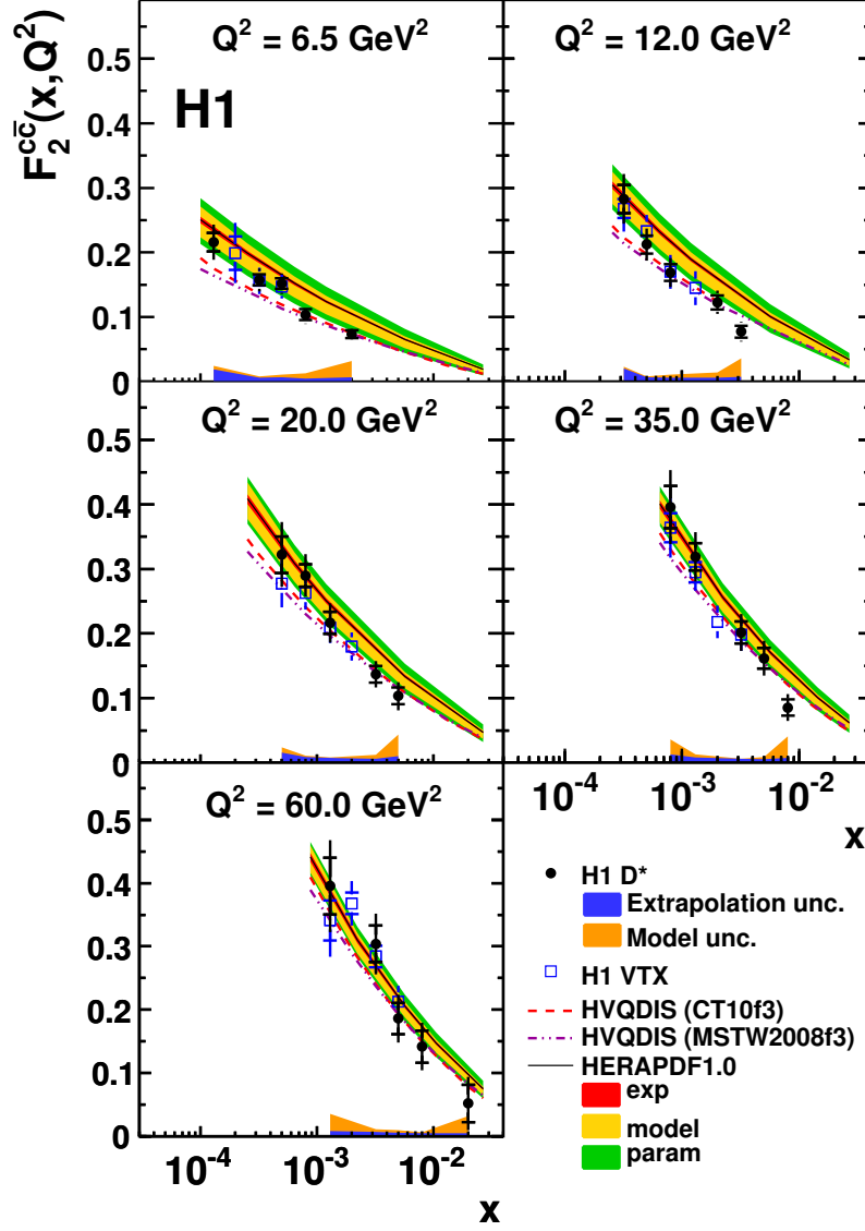
Figure 16: F_2^{c\bar{c}} as derived from D^* data with HVQDIS (points). The inner error bars show the statistical uncertainty, the outer error bar the statistical and experimental systematic uncertainty added in quadrature. The extrapolation uncertainty within the HVQDIS model is shown as blue band in the bottom of the plots. The outer (orange) band shows the model uncertainty obtained from the difference in F_2^{c\bar{c}} determined with HVQDIS and CASCADE. The data are compared to the measurement of F_2^{c\bar{c}} with the H1 vertex detector [14] (open squares), to NLO DGLAP predictions from HVQDIS with two different proton PDFs, and to the F_2^{c\bar{c}} prediction of HERAPDF1.0.
