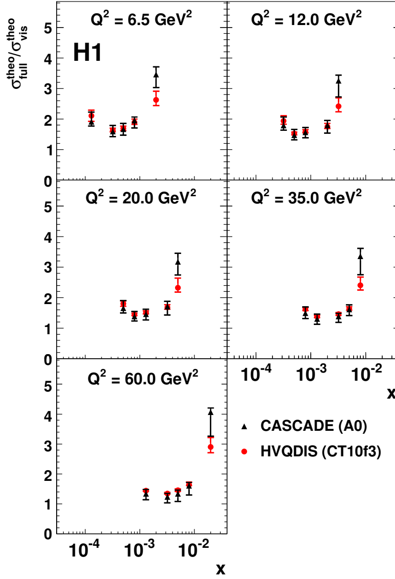
Figure 15: Extrapolation factors from the visible phase space (table 3) to the total phase space for the D^* meson as determined from HVQDIS and CASCADE. The error bars show the extrapolation uncertainty which is determined by varying the theory parameters listed in table 2 for HVQDIS and in table 1 for CASCADE.
