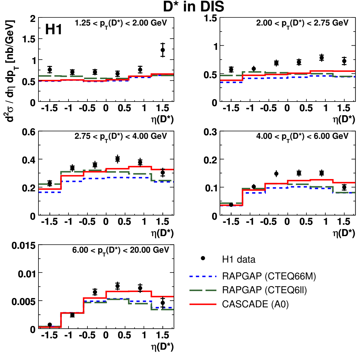
Figure 6: Double differential D^* cross section as a function of the transverse momentum p_T(D^*) and pseudo-rapidity \eta(D^*) in the laboratory frame. The measurements correspond to the kinematic range of 5 < Q^2 < 100 GeV 2 , 0.02 < y < 0.7 and |\eta(D^*)| < 1.8 and p_T(D^*) > 1.25 GeV. The data are shown as points, the inner error bars show the statistical error, the outer error bars represent the statistical and systematic errors added in quadrature. The data are compared to predictions by the MC program RAPGAP with two different proton parton densities and by the MC program CASCADE.
