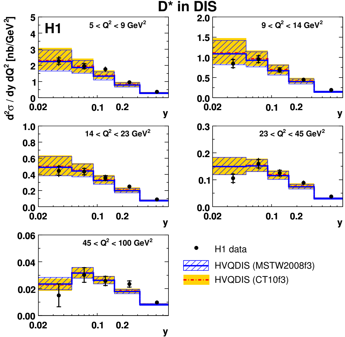
Figure 11: Double differential D^* cross section as a function of photon virtuality Q^2 and the inelasticity y . The measurements correspond to the kinematic range of 5 < Q^2 < 100 \text{ GeV}^2 , 0.02 < y < 0.7 and |\eta(D^*)| < 1.8 and p_T(D^*) > 1.25 \text{ GeV} . The data are shown as points, the inner error bars show the statistical error, the outer error bars represent the statistical and systematic errors added in quadrature. The data are compared to predictions by the next-to-leading order calculation HVQDIS with two different proton parton densities. The bands indicate the theoretical uncertainties (table 2).
