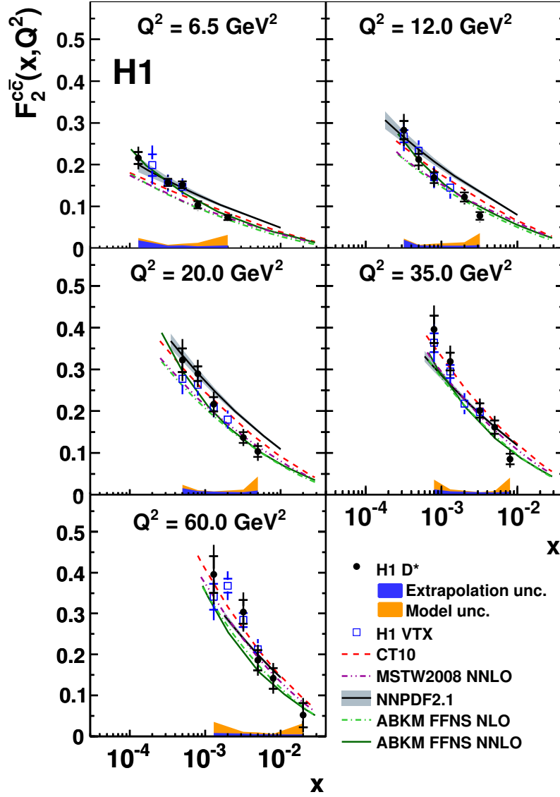
Figure 17: F_2^{cc} as derived from D^* data with HVQDIS (points). The inner error bars show the statistical uncertainty, the outer error bar the statistical and experimental systematic uncertainty added in quadrature. The extrapolation uncertainty within the HVQDIS model is shown as blue band in the bottom of the plots. The outer (orange) band shows the model uncertainty obtained from the difference in F_2^{cc} determined with HVQDIS and CASCADE. The data are compared to the measurement of F_2^{cc} with the H1 vertex detector [14] (open squares) and to predictions from the global PDF fits CT10 (dashed line), MSTW08 at NNLO (dark dashed-dotted line), NNPDF2.1 (shaded band) and ABKM at NLO (light dashed-dotted line) and NNLO (solid line).
