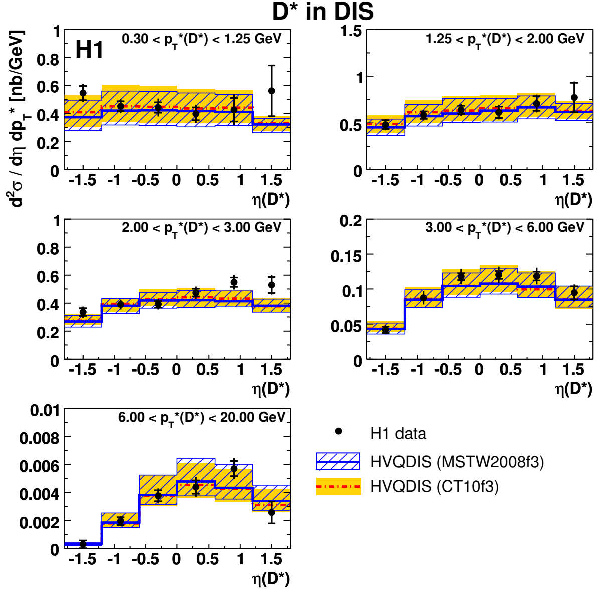
Figure 9: Double differential D^* cross section as a function of the transverse momentum in the \gamma p centre-of-mass frame p_T^*(D^*) and the pseudo-rapidity \eta(D^*) in the laboratory frame. The measurements correspond to the kinematic range of 5 < Q^2 < 100 GeV 2 , 0.02 < y < 0.7 and |\eta(D^*)| < 1.8 and p_T(D^*) > 1.25 GeV. The data are shown as points, the inner error bars show the statistical error, the outer error bars represent the statistical and systematic errors added in quadrature. The data are compared to predictions by the next-to-leading order calculation HVQDIS with two different proton parton densities. The bands indicate the theoretical uncertainties (table 2).
