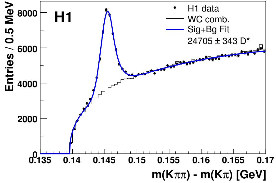
Figure 1: Distribution of the mass difference \Delta m = m(K^\pm \pi^\pm \pi_s^\pm) - m(K^\pm \pi^\pm) for D^* candidates in the kinematic range of 5 < Q^2 < 100 \text{ GeV}^2 , 0.02 < y < 0.7 , |\eta(D^*)| < 1.8 and p_T(D^*) > 1.25 \text{ GeV} . The histogram shows the wrong charge combinations, K^\pm \pi^\pm \pi_s^\mp . The solid line represents the result of the fit described in the text.
