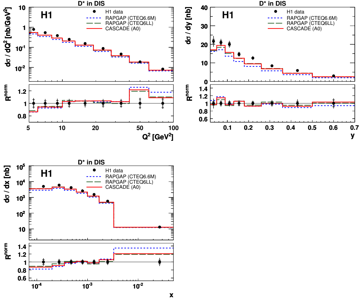
Figure 2: Differential D^* cross section as a function of the photon virtuality Q^2 , the inelasticity y and Bjorken x . The measurements correspond to the kinematic range of 5 < Q^2 < 100 \text{ GeV}^2 , 0.02 < y < 0.7 , |\eta(D^*)| < 1.8 and p_T(D^*) > 1.25 \text{ GeV} . The data are shown as points, the inner error bars show the statistical error, the outer error bars represent the statistical and systematic errors added in quadrature. The data are compared to predictions by the MC program RAPGAP with two different proton parton densities and by the MC program CASCADE. In the lower part of the figures the normalised ratio R^{\text{norm}} of theory to data (equation 3) is shown, which has reduced normalisation uncertainties.
