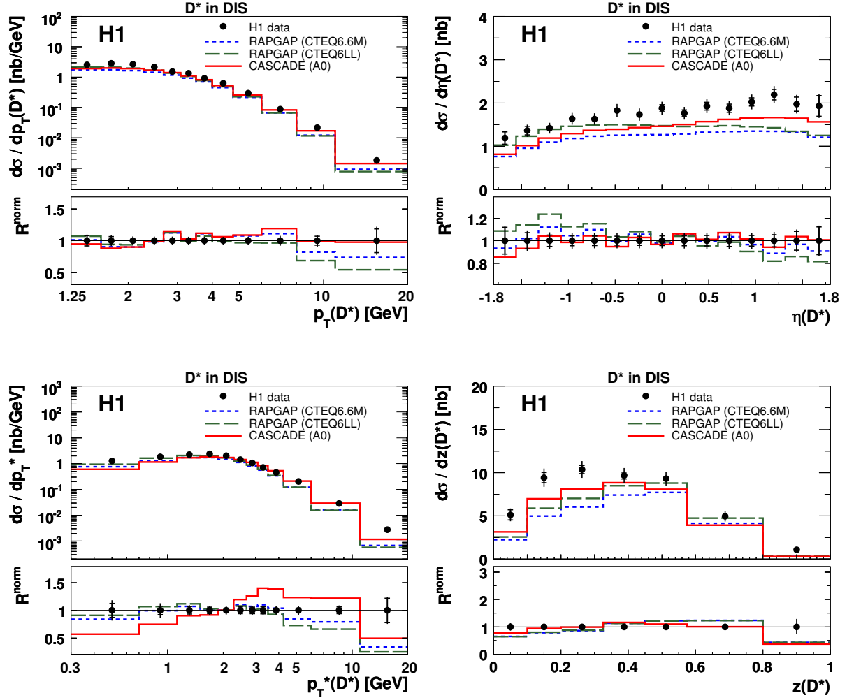
Figure 4: Differential D^* cross section as a function of the transverse momentum p_T(D^*) and pseudo-rapidity \eta(D^*) in the laboratory frame, the transverse momentum p_T^*(D^*) in the \gamma p centre-of-mass frame and the D^* inelasticity z(D^*) . The measurements correspond to the kinematic range of 5 < Q^2 < 100 \text{ GeV}^2 , 0.02 < y < 0.7 and |\eta(D^*)| < 1.8 and p_T(D^*) > 1.25 \text{ GeV} . The data are shown as points, the inner error bars show the statistical error, the outer error bars represent the statistical and systematic errors added in quadrature. The data are compared to predictions by the MC program RAPGAP with two different proton parton densities and by the MC program CASCADE. In the lower part of the figures the normalised ratio R^{\text{norm}} of theory to data (equation 3) is shown, which has reduced normalisation uncertainties.
