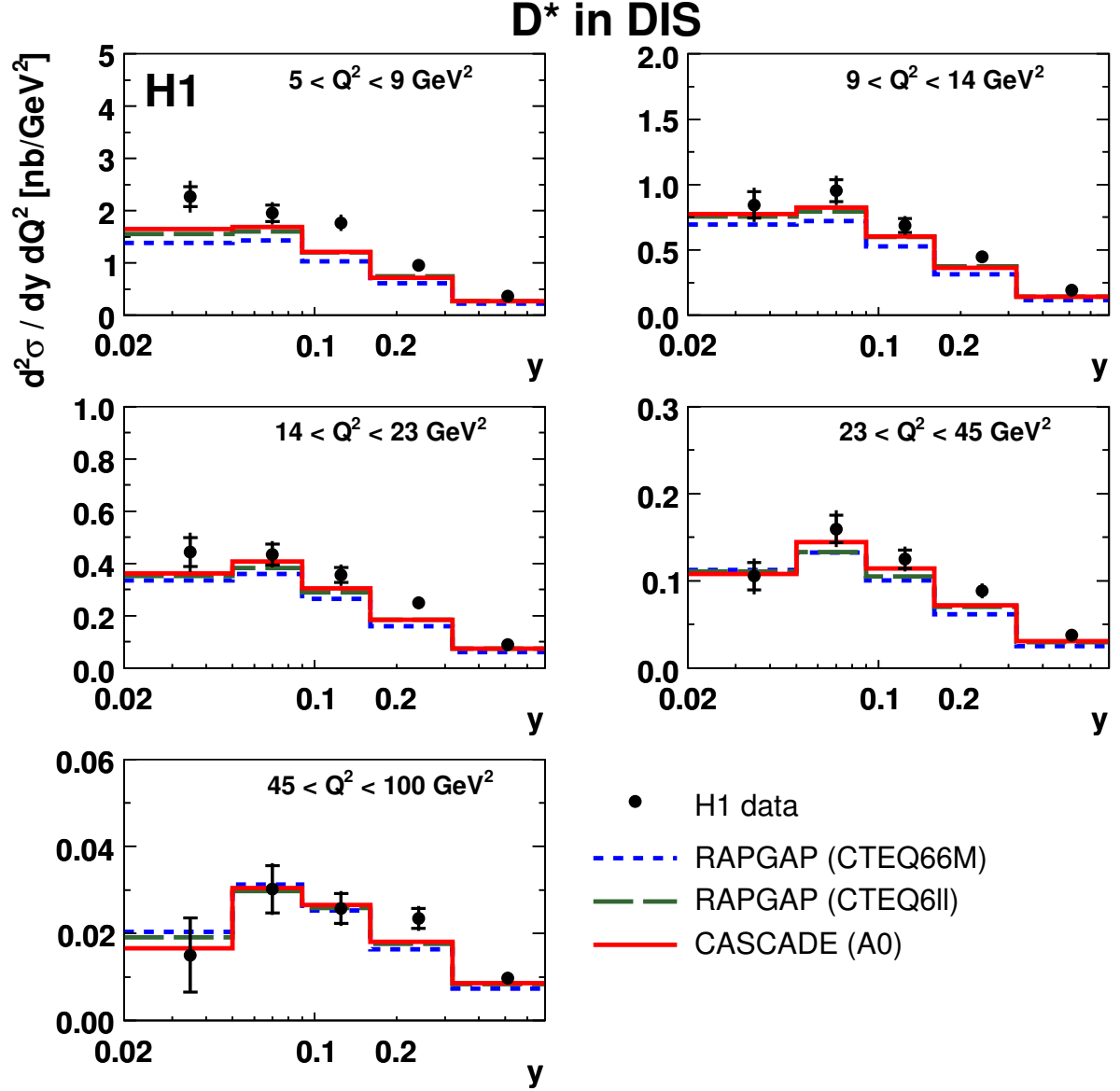
Figure 10: Double differential D^* cross section as a function of the photon virtuality Q^2 and the inelasticity y . The measurements correspond to the kinematic range of 5 < Q^2 < 100 \text{ GeV}^2 , 0.02 < y < 0.7 and |\eta(D^*)| < 1.8 and p_T(D^*) > 1.25 \text{ GeV} . The data are shown as points, the inner error bars show the statistical error, the outer error bars represent the statistical and systematic errors added in quadrature. The data are compared to predictions by the MC program RAPGAP with two different proton parton densities and by the MC program CASCADE.
