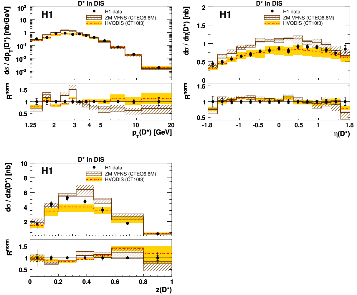
Figure 13: Differential D^* cross section as a function of the transverse momentum p_T(D^*) and pseudo-rapidity \eta(D^*) in the laboratory frame and the D^* inelasticity z(D^*) . The measurements correspond to the kinematic range of 5 < Q^2 < 100 \text{ GeV}^2 , 0.02 < y < 0.7 , |\eta(D^*)| < 1.8 , p_T(D^*) > 1.25 \text{ GeV} with an additional cut on the D^* transverse momentum in the \gamma p centre-of-mass frame p_T^*(D^*) > 2.0 \text{ GeV} . The data are shown as points, the inner error bars show the statistical error, the outer error bars represent the statistical and systematic errors added in quadrature. The data are compared to a prediction to next-to-leading order in the ZM-VFNS and to HVQDIS. The bands indicate the theoretical uncertainties (table 2).
