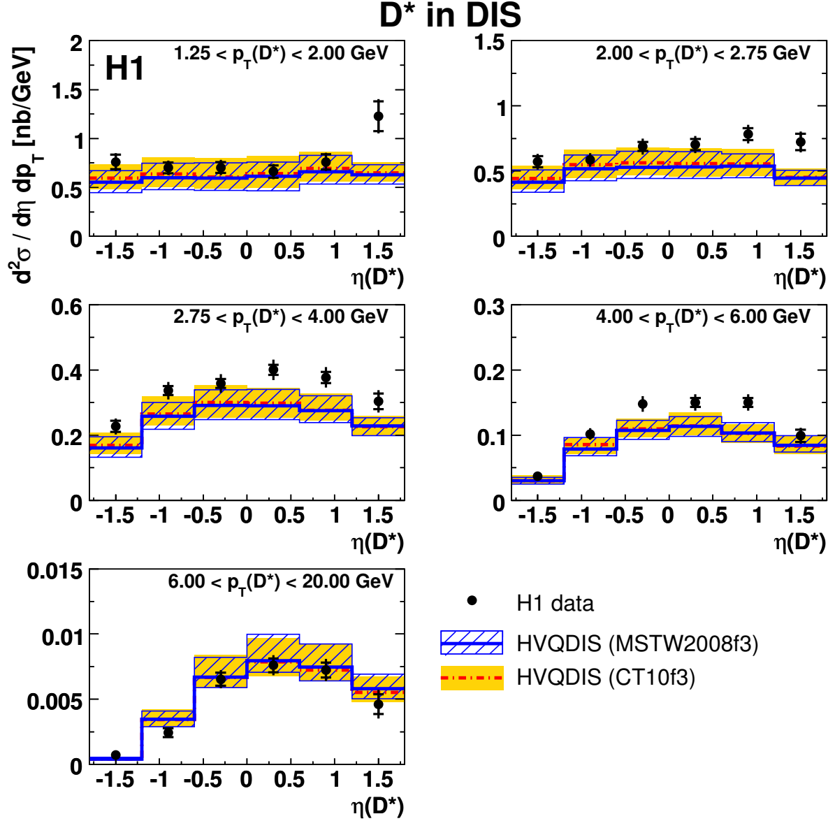
Figure 7: Double differential D^* cross section as a function of the transverse momentum p_T(D^*) and pseudo-rapidity \eta(D^*) in the laboratory frame. The measurements correspond to the kinematic range of 5 < Q^2 < 100 \text{ GeV}^2 , 0.02 < y < 0.7 and |\eta(D^*)| < 1.8 and p_T(D^*) > 1.25 \text{ GeV} . The data are shown as points, the inner error bars show the statistical error, the outer error bars represent the statistical and systematic errors added in quadrature. The data are compared to predictions by the next-to-leading order calculation HVQDIS with two different proton parton densities. The bands indicate the theoretical uncertainties (table 2).
