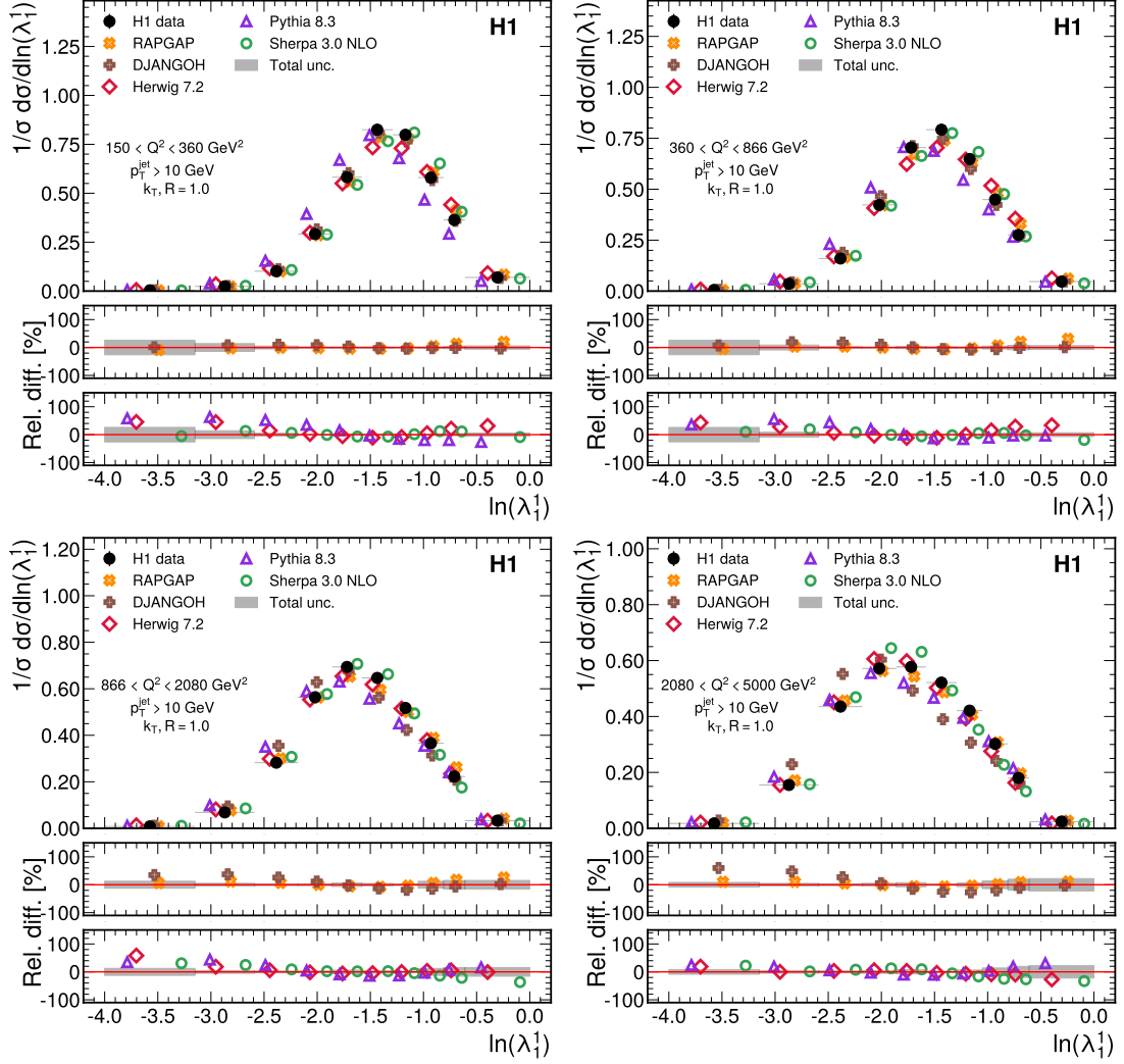
Fig. 5 Measured cross sections, normalized to the inclusive jet production cross section, for multiple Q^2 intervals as a function of \ln(\lambda_1^1) . Data are shown as solid dots, horizontal bars indicate the bin ranges. Predictions from multiple simulations are shown for comparison, and are offset horizontally for visual clarity. The relative differences between data and predictions are shown in the bottom panels, split between dedicated DIS simulators (middle) and general purpose simulators (bottom). Gray bands represent the total data uncertainties.
