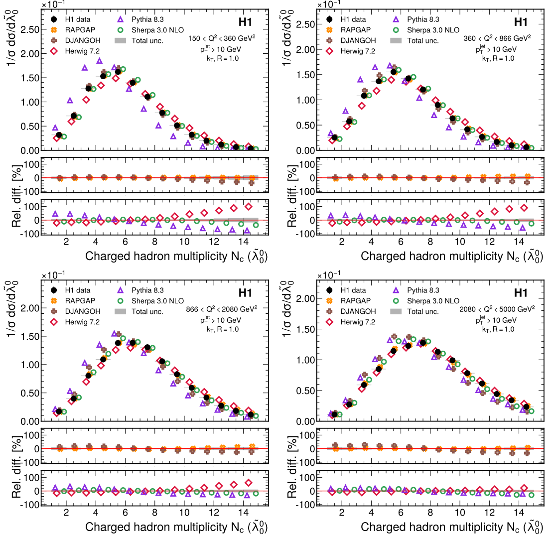
Fig. 10 Measured cross sections, normalized to the inclusive jet production cross section, for multiple Q^2 intervals as a function of N_c . Data are shown as solid dots, horizontal bars indicate the bin ranges. Predictions from multiple simulations are shown for comparison, and are offset horizontally for visual clarity. The relative differences between data and predictions are shown in the bottom panels, split between DIS simulators (middle) and general purpose simulators (bottom). Gray bands represent the total data uncertainties.
