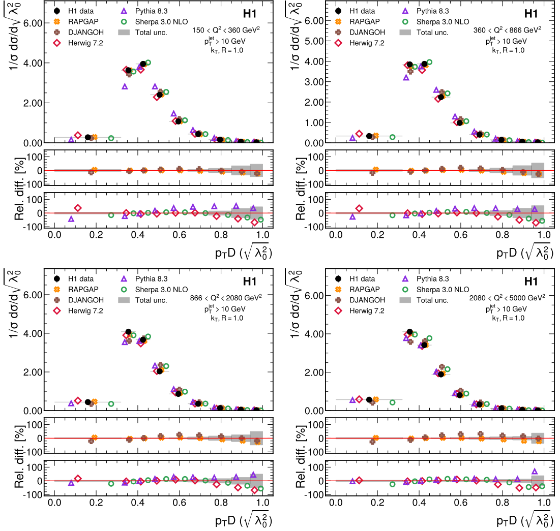
Fig. 8 Measured cross sections, normalized to the inclusive jet production cross section, for multiple Q^2 intervals (columns) as a function of p_{TD} . Data are shown as solid dots, horizontal bars indicate the bin ranges. Predictions from multiple simulations are shown for comparison, and are offset horizontally for visual clarity. The relative differences between data and predictions are shown in the bottom panels, split between dedicated DIS simulators (middle) and general purpose simulators (bottom). Gray bands represent the total data uncertainties.
