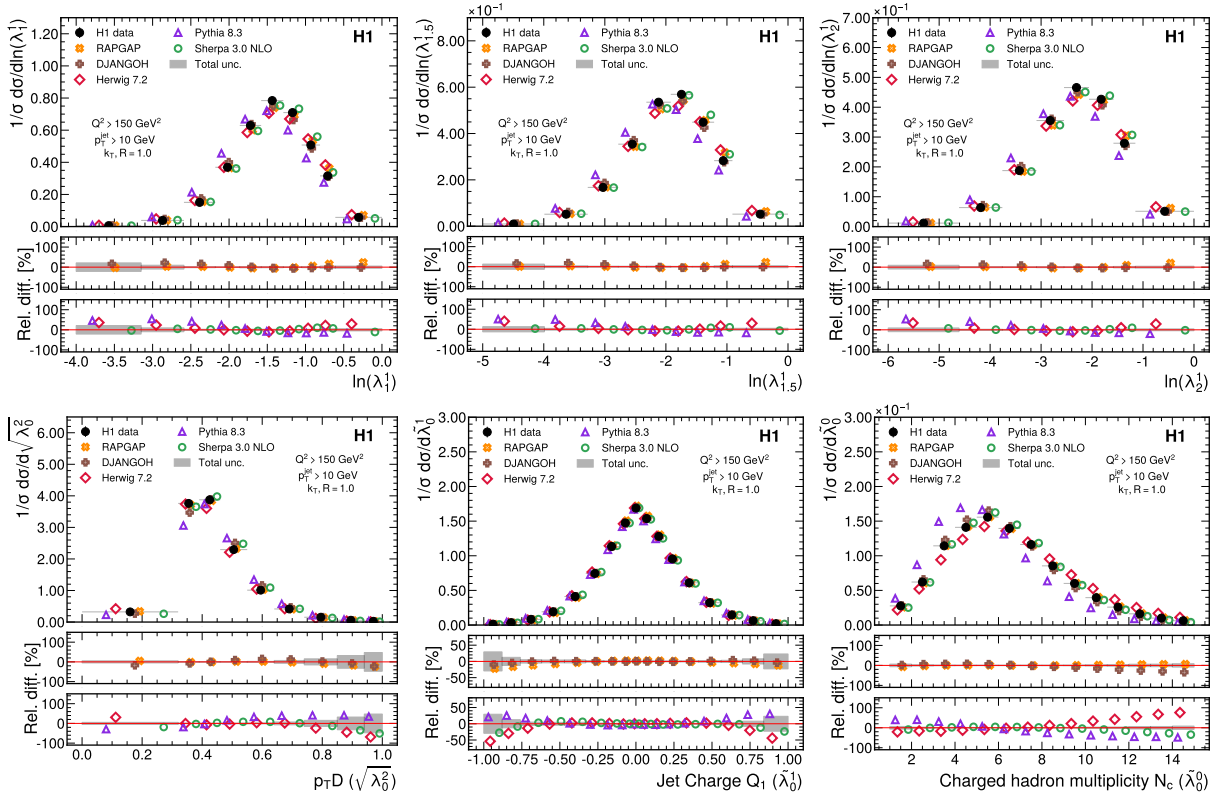
Figure 1: Measured cross sections, normalized to the inclusive jet production cross section as a function of the jet angularities measured in this work. Data are shown as solid dots, horizontal bars indicate the bin ranges. Predictions from multiple simulations are shown for comparison, and are offset horizontally for visual clarity. The relative differences between data and predictions are shown in the bottom panels, split between dedicated DIS simulators (middle) and general purpose simulators (bottom). Gray bands represent the total data uncertainties.
