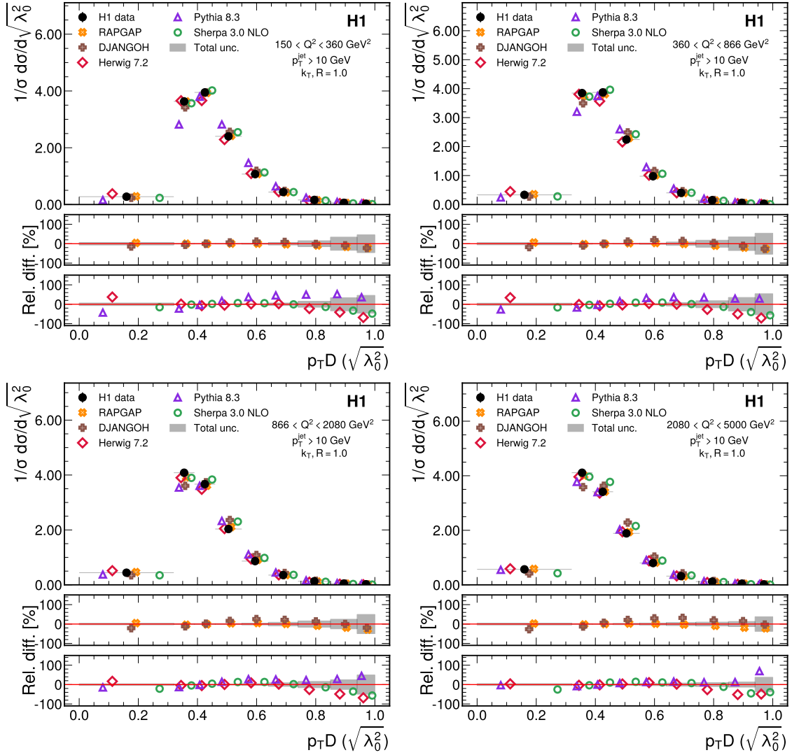
Figure B.8: Measured cross sections, normalized to the inclusive jet production cross section, for multiple Q^2 intervals (columns) as a function of p_{TD} . Data are shown as solid dots, horizontal bars indicate the bin ranges. Predictions from multiple simulations are shown for comparison, and are offset horizontally for visual clarity. The relative differences between data and predictions are shown in the bottom panels, split between dedicated DIS simulators (middle) and general purpose simulators (bottom). Gray bands represent the total data uncertainties.
