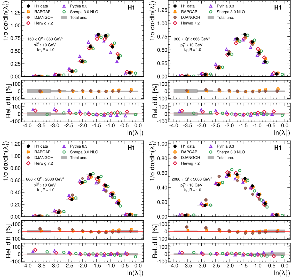
Figure B.5: Measured cross sections, normalized to the inclusive jet production cross section, for multiple Q^2 intervals as a function of \ln(\lambda_1^1) . Data are shown as solid dots, horizontal bars indicate the bin ranges. Predictions from multiple simulations are shown for comparison, and are offset horizontally for visual clarity. The relative differences between data and predictions are shown in the bottom panels, split between dedicated DIS simulators (middle) and general purpose simulators (bottom). Gray bands represent the total data uncertainties.
