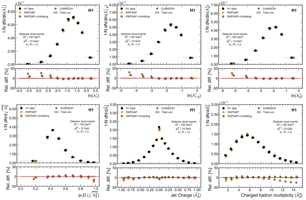
Figure A.4: Measured cross sections at reconstruction level, normalized to the inclusive jet production cross section, as a function of the jet angularities. Data are shown as solid dots, horizontal bars indicate the bin ranges. Predictions from DJANGO and RAPGAP simulations are shown for comparison, as well as RAPGAP predictions with unfolding weights. The predictions are offset horizontally for visual clarity. The relative differences between data and predictions are shown in the bottom panels. Gray bands represent the total systematic uncertainties from detector effects. Data statistical uncertainties are shown as vertical bars, while the statistical uncertainties on the simulations are smaller than the marker sizes.
