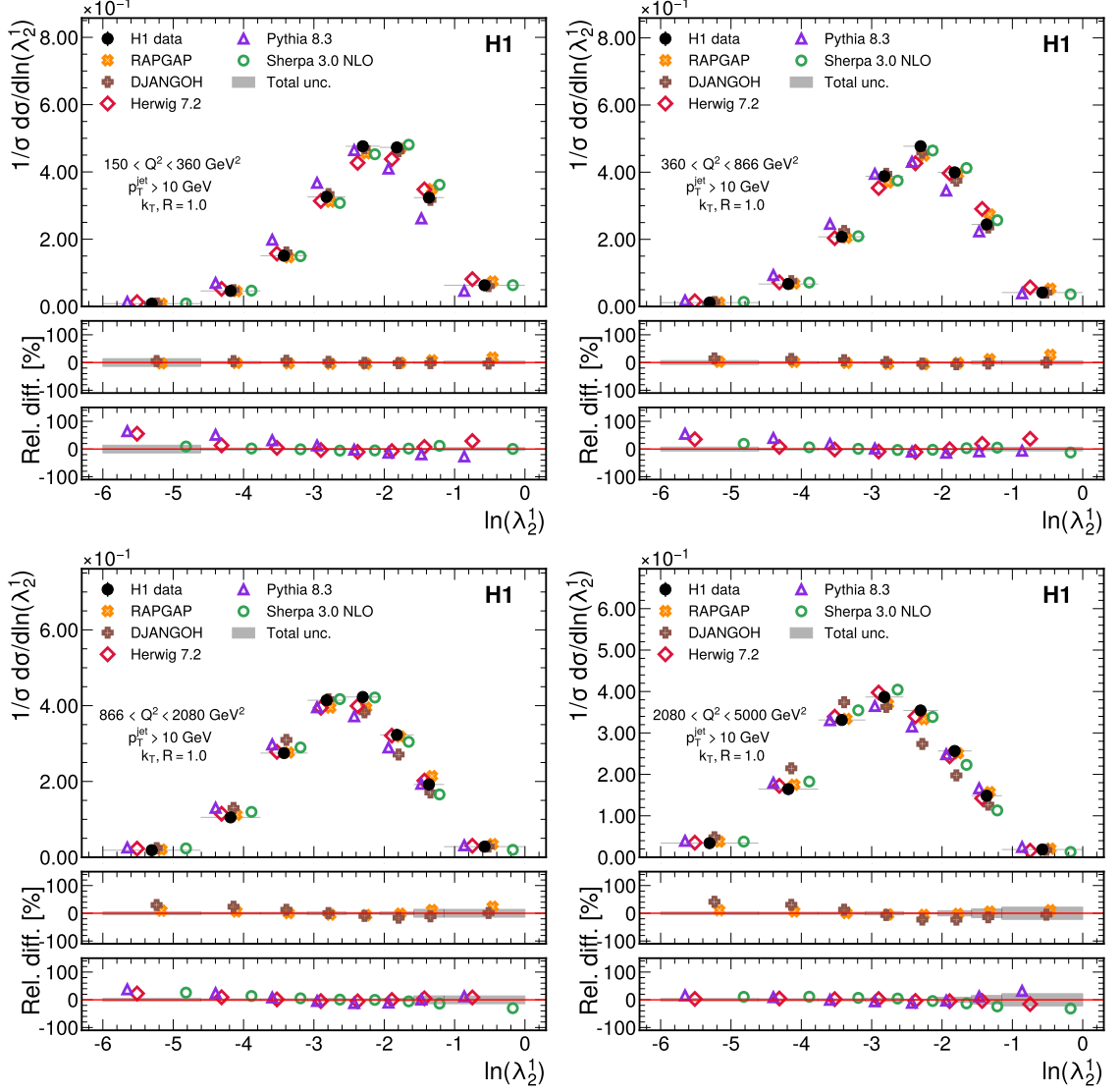
Figure B.7: Measured cross sections, normalized to the inclusive jet production cross section, for multiple Q^2 intervals as a function of \ln(\lambda_2^1) . Data are shown as solid dots, horizontal bars indicate the bin ranges. Predictions from multiple simulations are shown for comparison, and are offset horizontally for visual clarity. The relative differences between data and predictions are shown in the bottom panels, split between dedicated DIS simulators (middle) and general purpose simulators (bottom). Gray bands represent the total data uncertainties.
